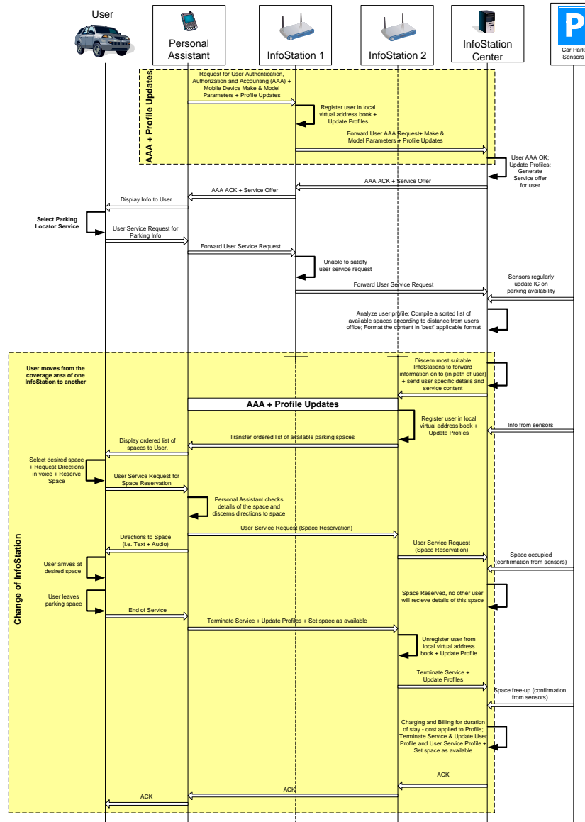
Figure 6: Intelligent Parking Locator Service: Entity Interactions
